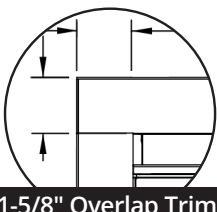
1-5/8" Overlap Trim
